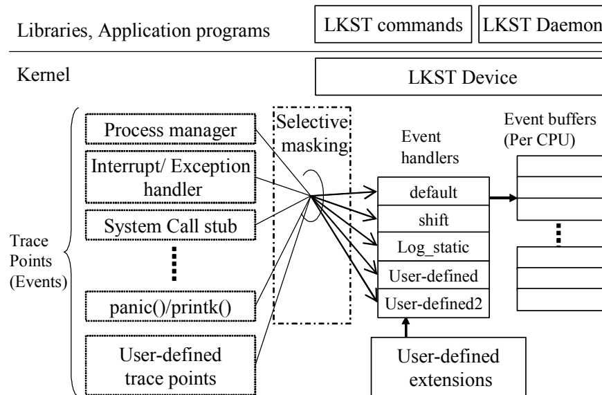
Figure 3-1 LKST block diagram.
