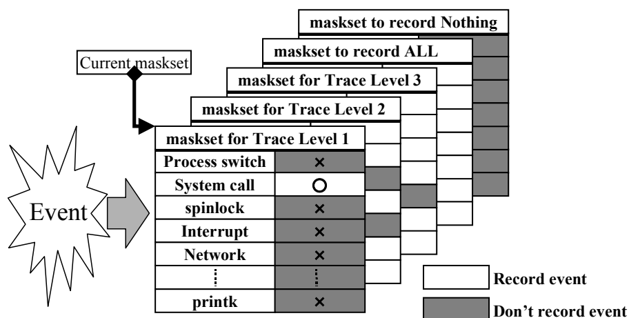
Figure 4-1. Masksets.
