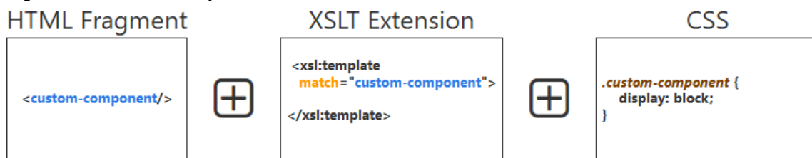
Figure 22. Custom Component
